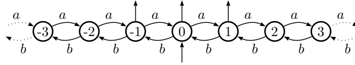
FIGURE 1. The minimal automaton of L .
